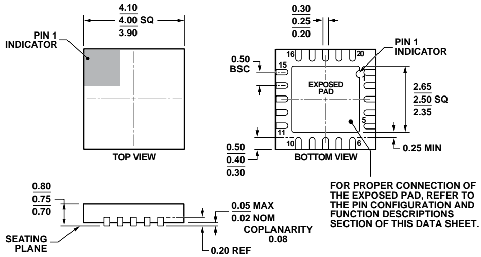
Figure 110. 20-Lead Lead Frame Chip Scale Package [LFCSP_WQ] 4 mm x 4 mm Body, Very Very Thin Quad (CP-20-10) Dimensions shown in millimeters
