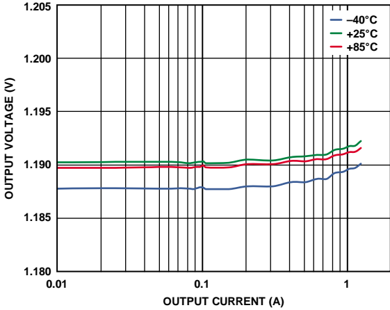
Figure 16. Buck Load Regulation Across Temperature, V_{OUT1} = 1.2V , PWM Mode
